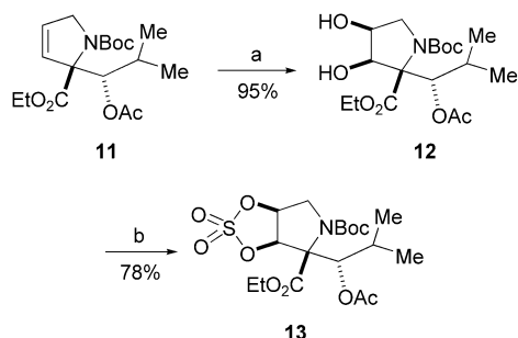
Scheme 4. Reagents and conditions: a) cat. \text{OsO}_4 , \text{Me}_3\text{NO} \cdot 2\text{H}_2\text{O} , \text{CH}_2\text{Cl}_2 ; b) 1. \text{SOCl}_2 , \text{Et}_3\text{N} , \text{CH}_2\text{Cl}_2 ; 2. cat. \text{RuCl}_3 \cdot x\text{H}_2\text{O} , \text{NaIO}_4 , \text{MeCN}/\text{CCl}_4/\text{H}_2\text{O} .
